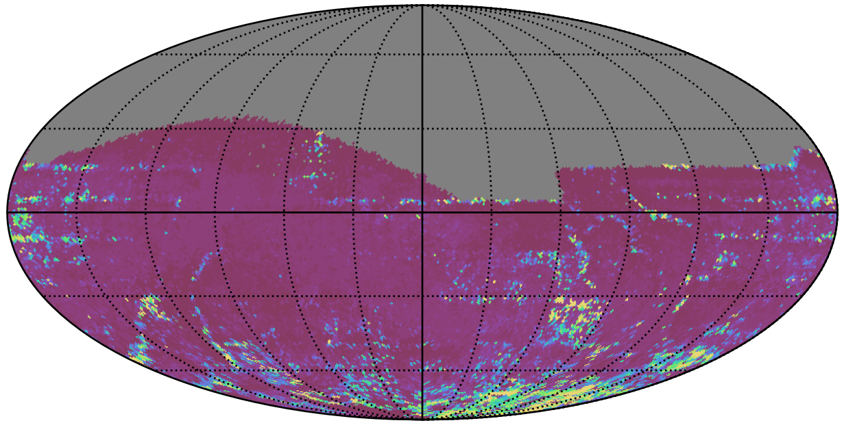
weather_cloudso16v3.4_10yrs All sky z band: 75th Percentile Intranight Timespan
