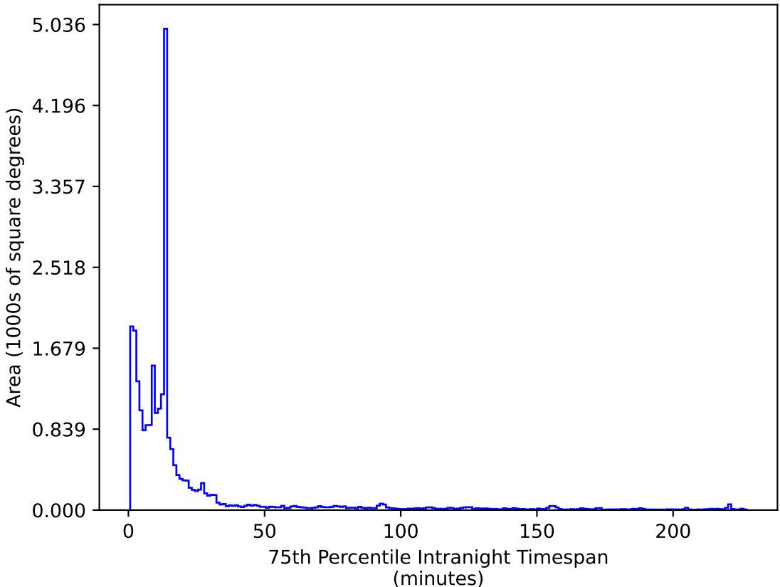
weather_cloudso16v3.4_10yrs All sky z band: 75th Percentile Intranight Timespan
