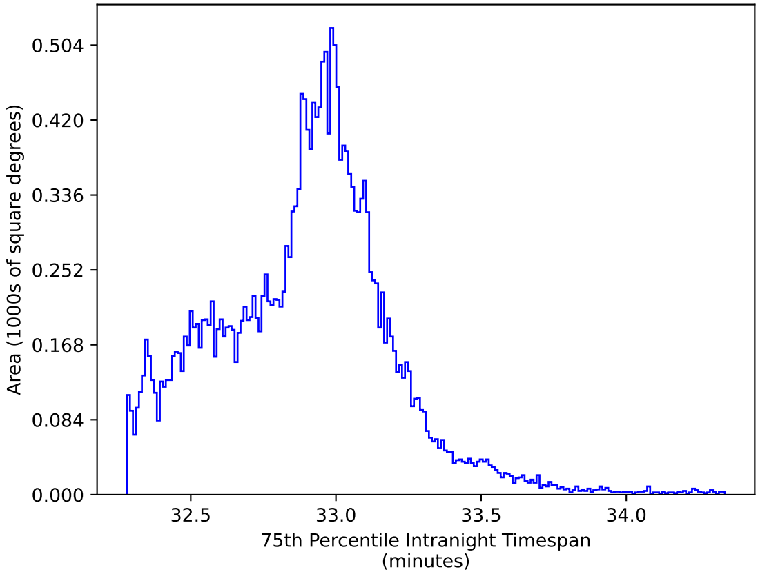
weather_cloudso16v3.4_10yrs All sky y band: 75th Percentile Intranight Timespan
