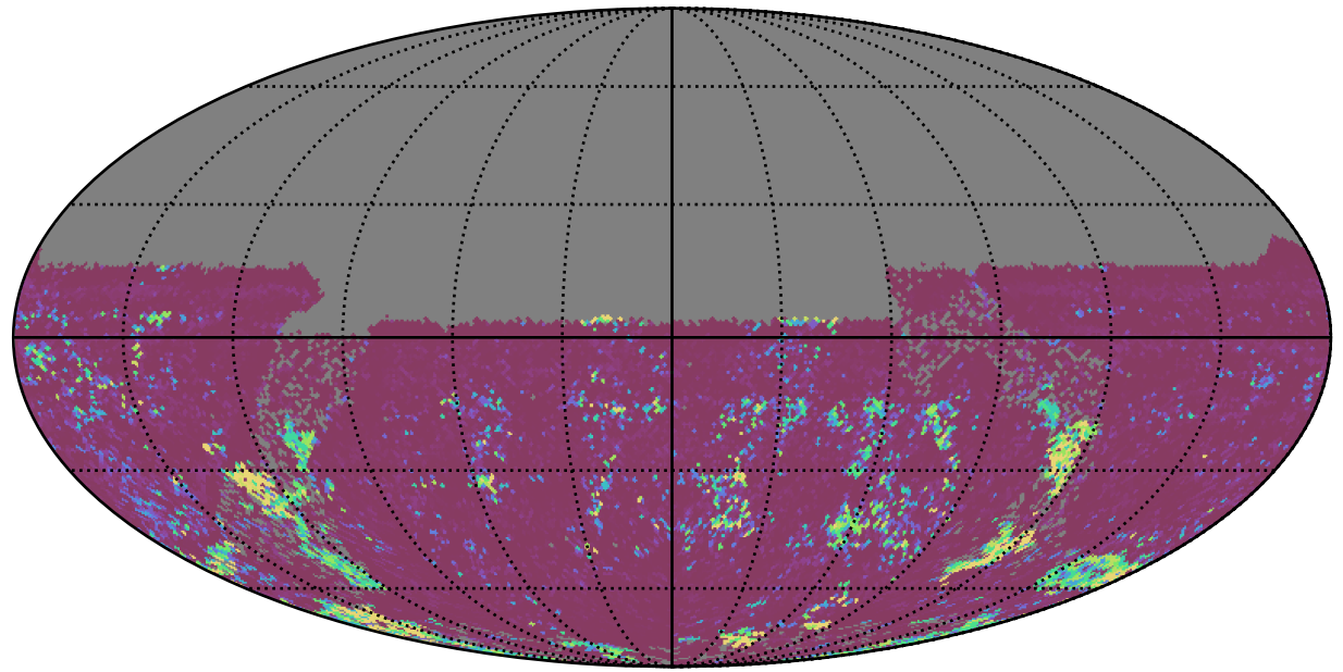
weather_cloudso16v3.4_10yrs All sky u band: 75th Percentile Intranight Timespan
