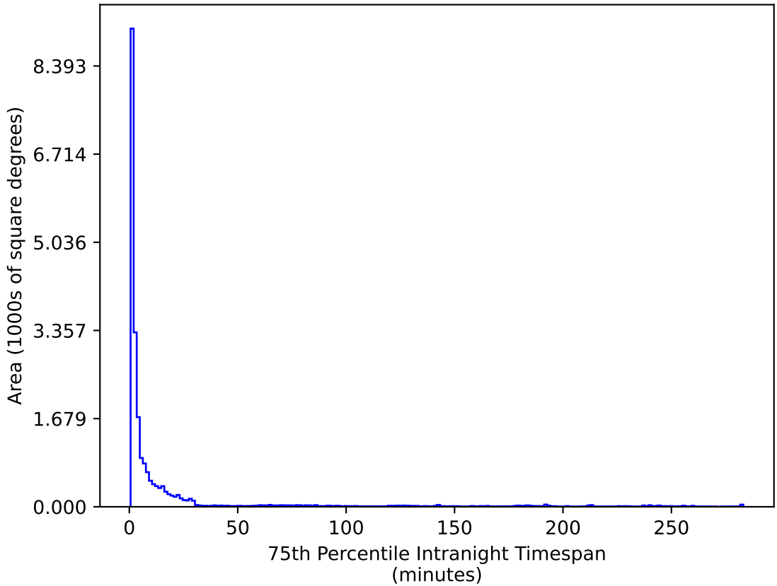
weather_cloudso16v3.4_10yrs All sky u band: 75th Percentile Intranight Timespan
