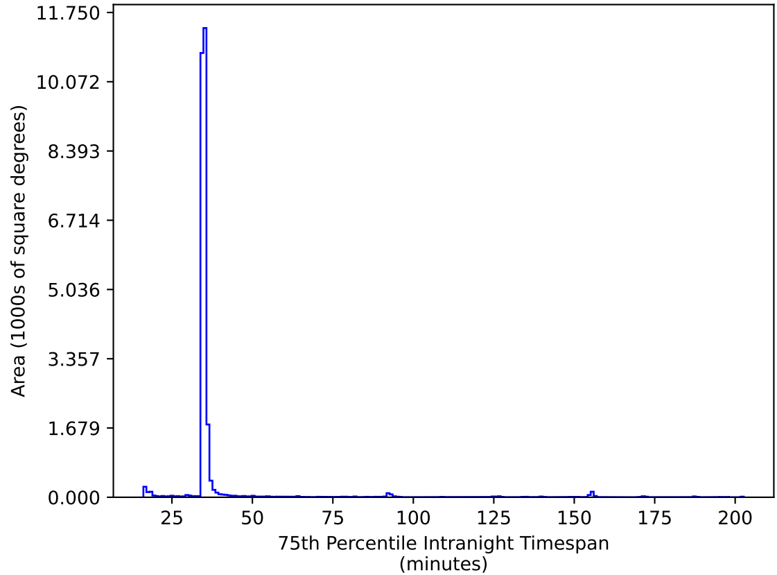
weather_cloudso16v3.4_10yrs All sky ri bands: 75th Percentile Intranight Timespan
