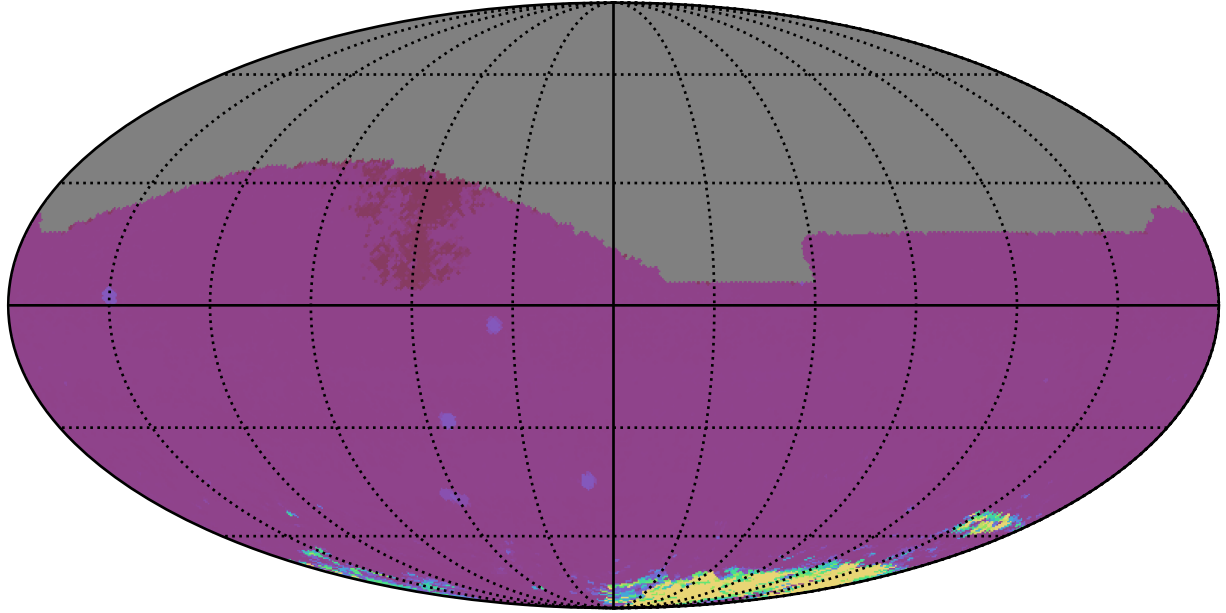
weather_cloudso16v3.4_10yrs All sky iz bands: 75th Percentile Intranight Timespan
