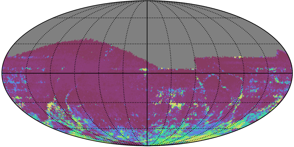
weather_cloudso16v3.4_10yrs All sky i band: 75th Percentile Intranight Timespan
