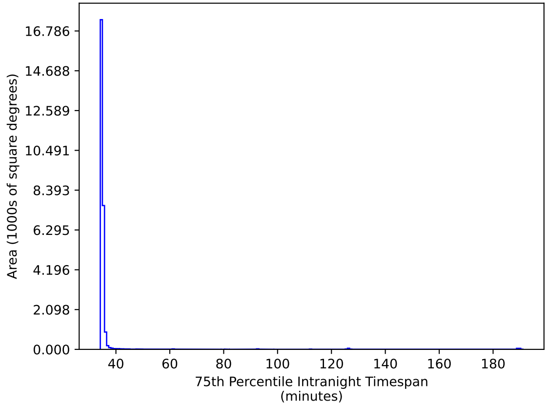
weather_cloudso16v3.4_10yrs All sky gr bands: 75th Percentile Intranight Timespan
