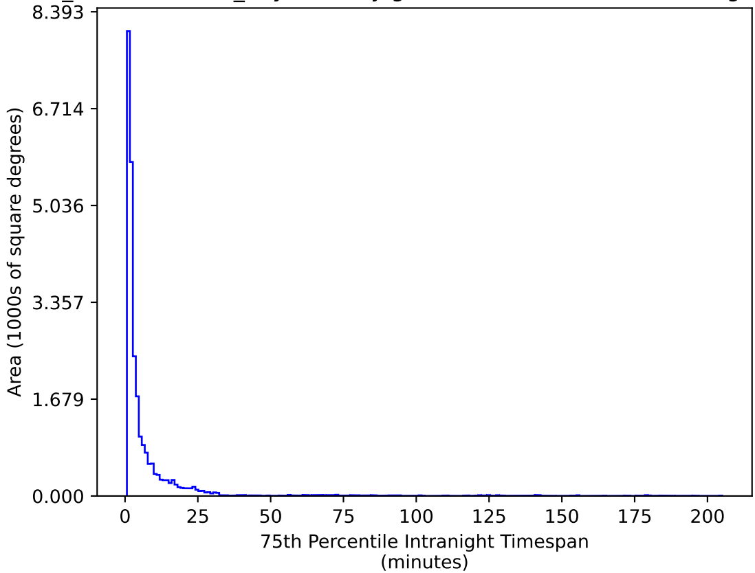
weather_cloudso16v3.4_10yrs All sky g band: 75th Percentile Intranight Timespan
