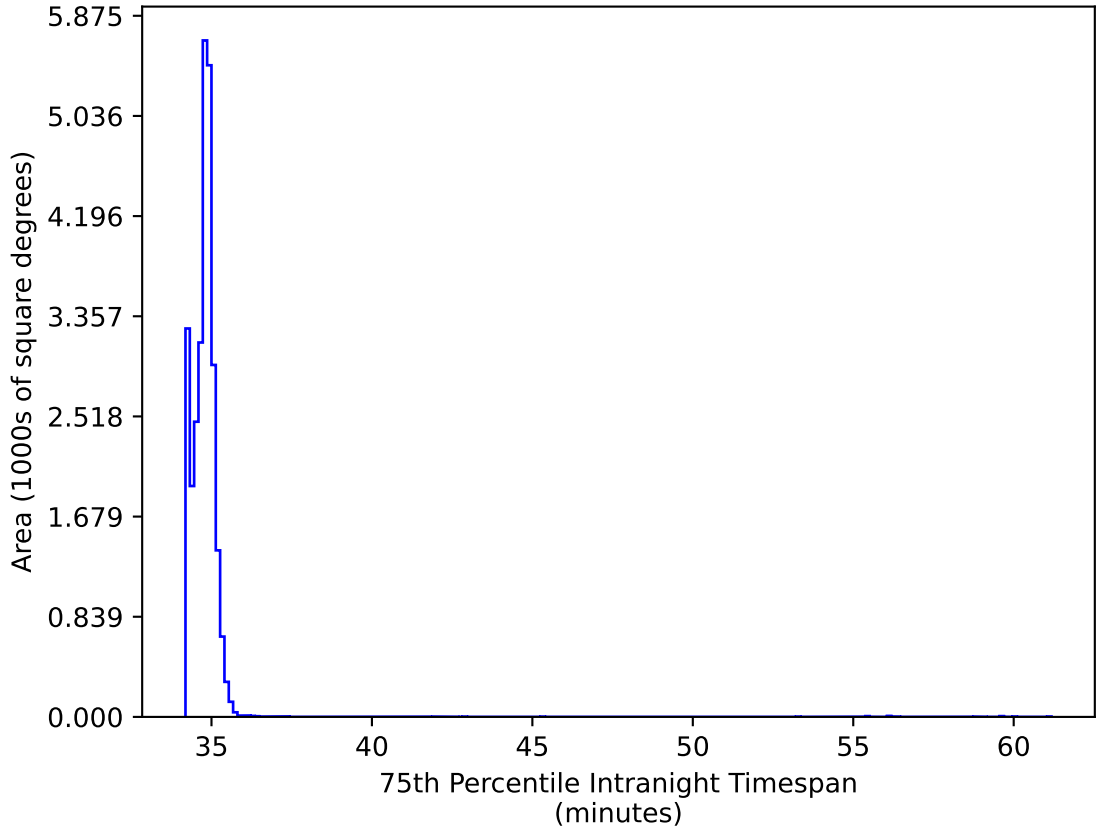
weather_cloudso16v3.4_10yrs All sky all bands: 75th Percentile Intranight Timespan
