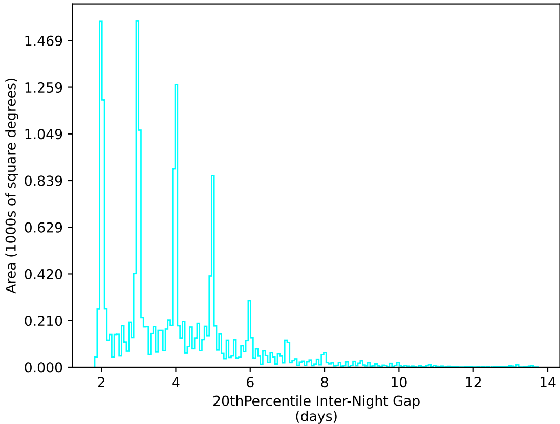
weather_cloudso16v3.4_10yrs WFD u band: 20thPercentile Inter-Night Gap
