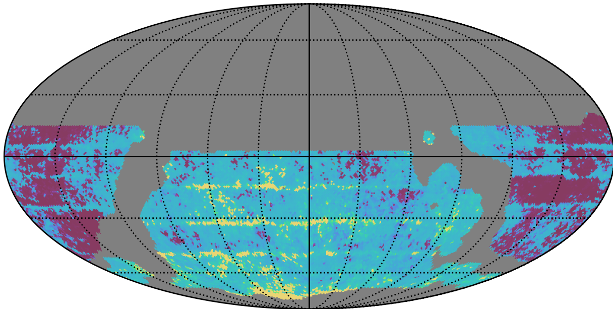
weather_cloudso16v3.4_10yrs WFD r band: 20thPercentile Inter-Night Gap
