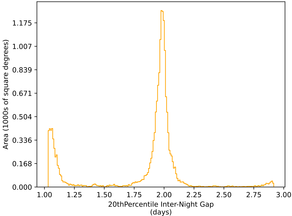
weather_cloudso16v3.4_10yrs WFD r band: 20thPercentile Inter-Night Gap
