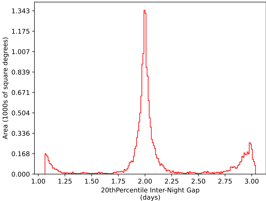
weather_cloudso16v3.4_10yrs WFD i band: 20thPercentile Inter-Night Gap
