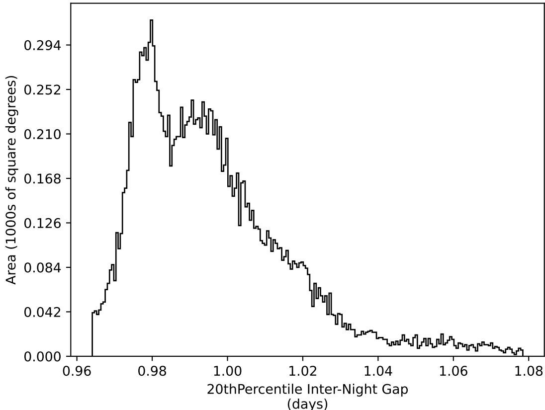
weather_cloudso16v3.4_10yrs WFD all bands: 20thPercentile Inter-Night Gap
