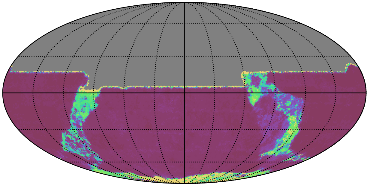
weather_cloudso16v3.4_10yrs All sky y band: 20thPercentile Inter-Night Gap
