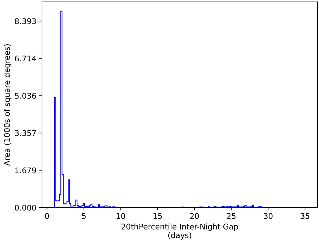
weather_cloudso16v3.4_10yrs All sky y band: 20thPercentile Inter-Night Gap
