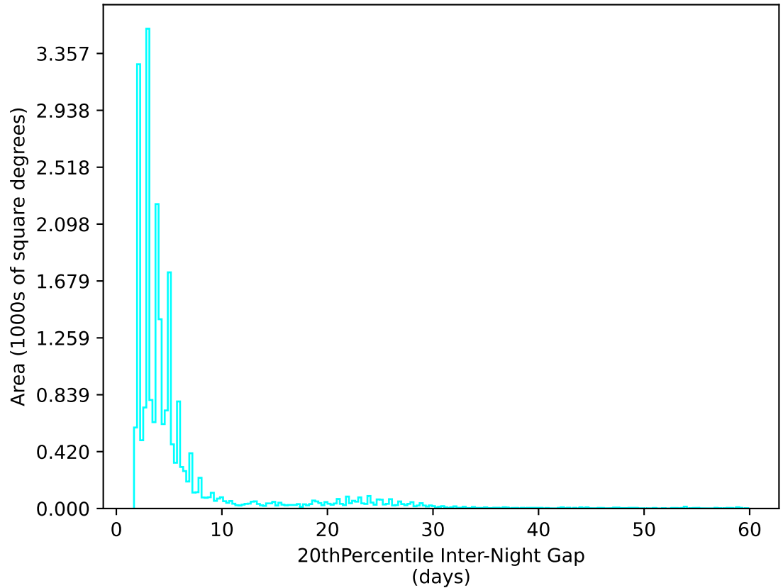
weather_cloudso16v3.4_10yrs All sky u band: 20thPercentile Inter-Night Gap
