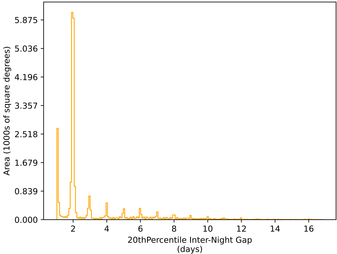
weather_cloudso16v3.4_10yrs All sky r band: 20thPercentile Inter-Night Gap
