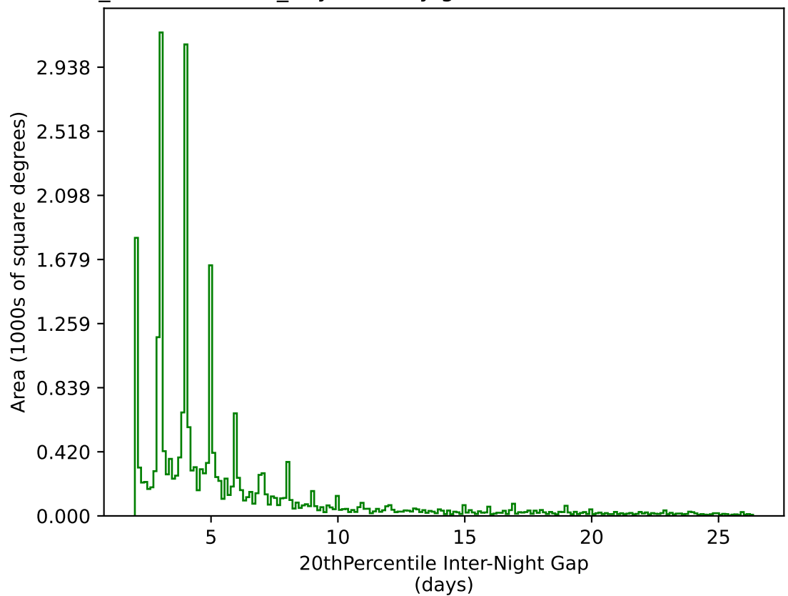
weather_cloudso16v3.4_10yrs All sky g band: 20thPercentile Inter-Night Gap
