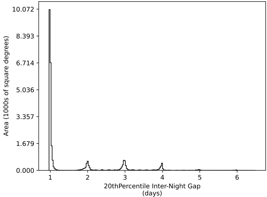
weather_cloudso16v3.4_10yrs All sky all bands: 20thPercentile Inter-Night Gap
