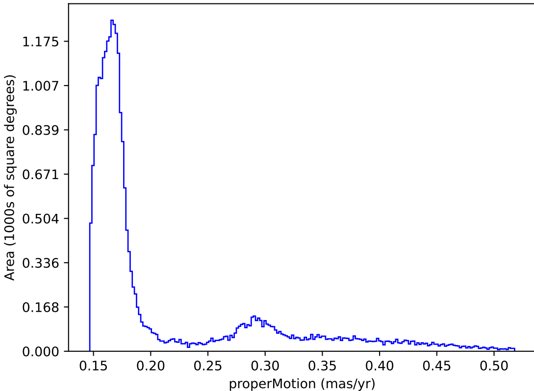
weather_cloudso16v3.4_10yrs : properMotion
