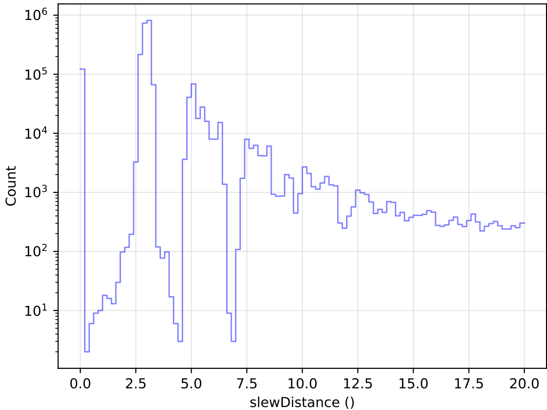
weather_cloudso16v3.4_10yrs All visits: Zoom Slew Distance Histogram
