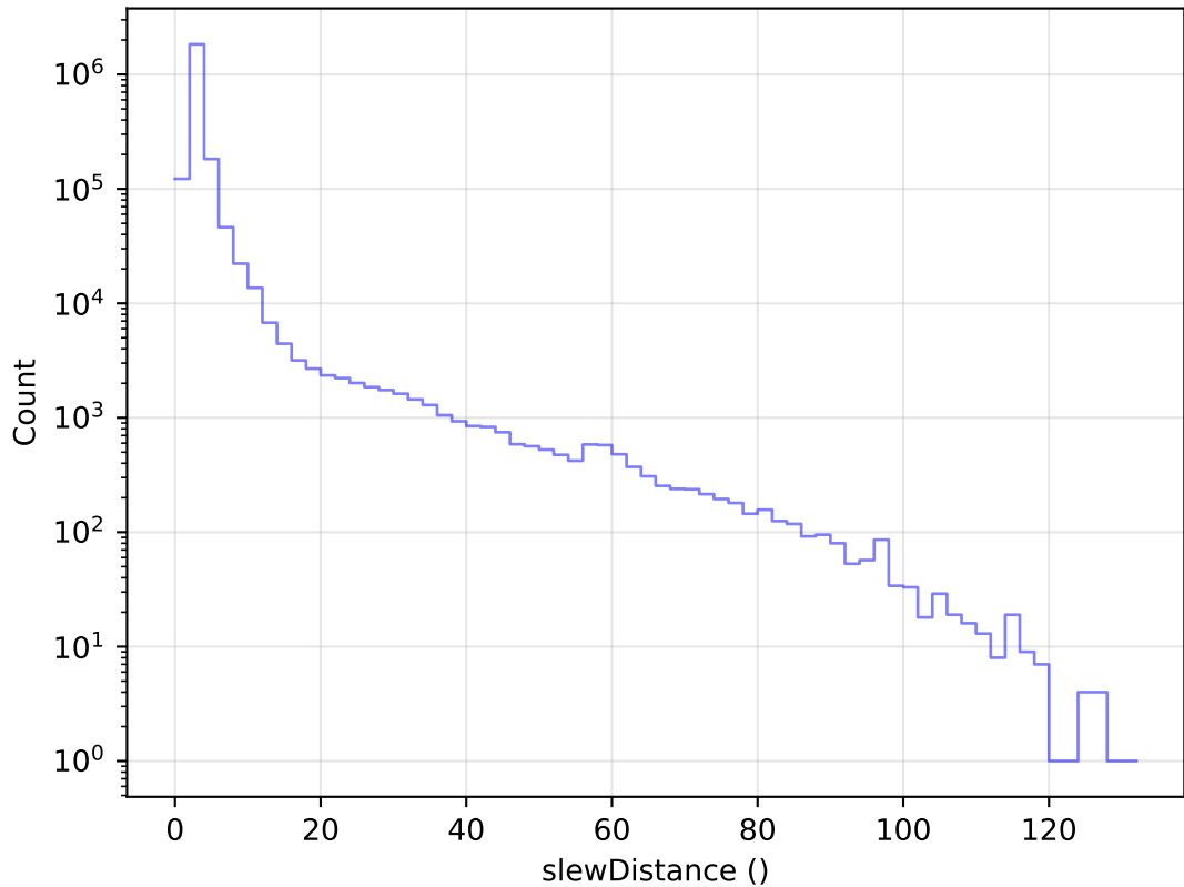
weather_cloudso16v3.4_10yrs All visits: Slew Distance Histogram
