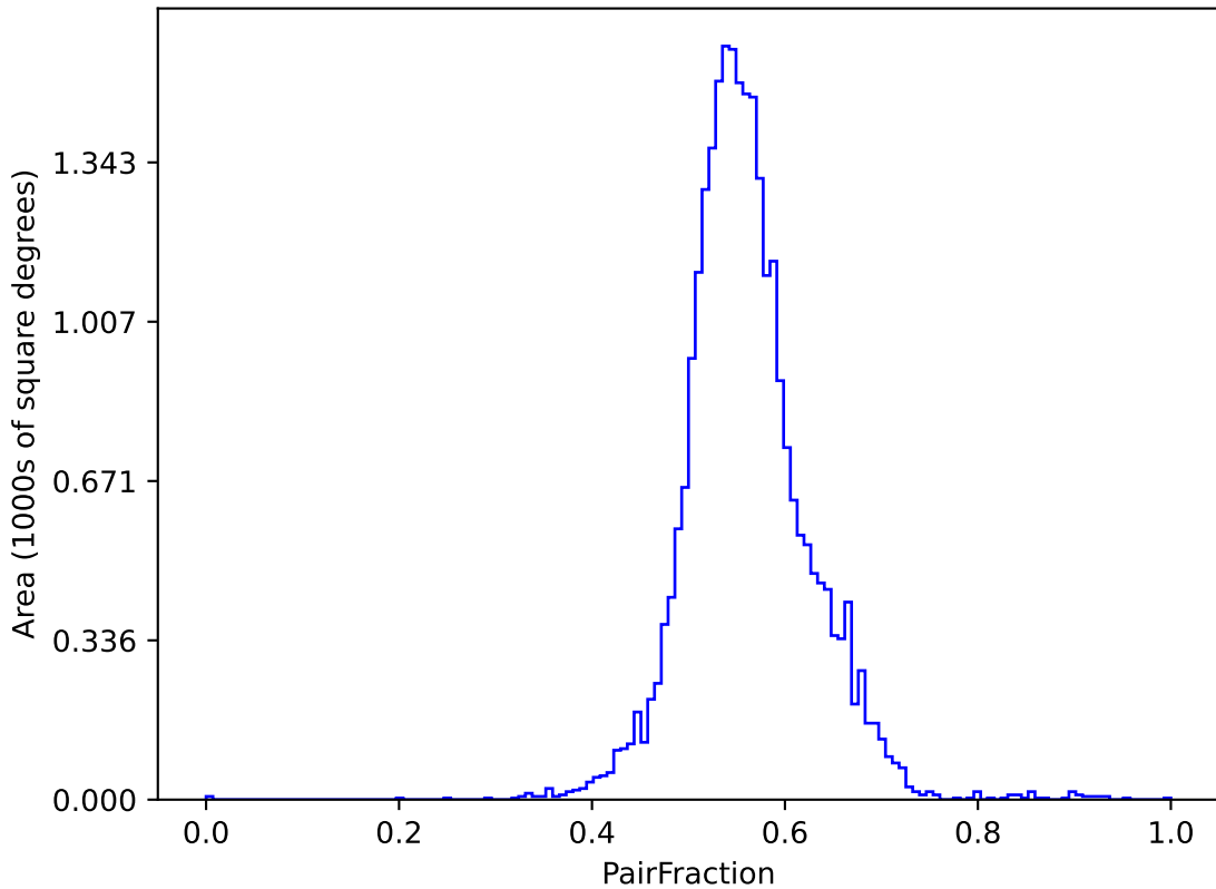
weather_cloudso16v3.4_10yrs (g or r or i): PairFraction
