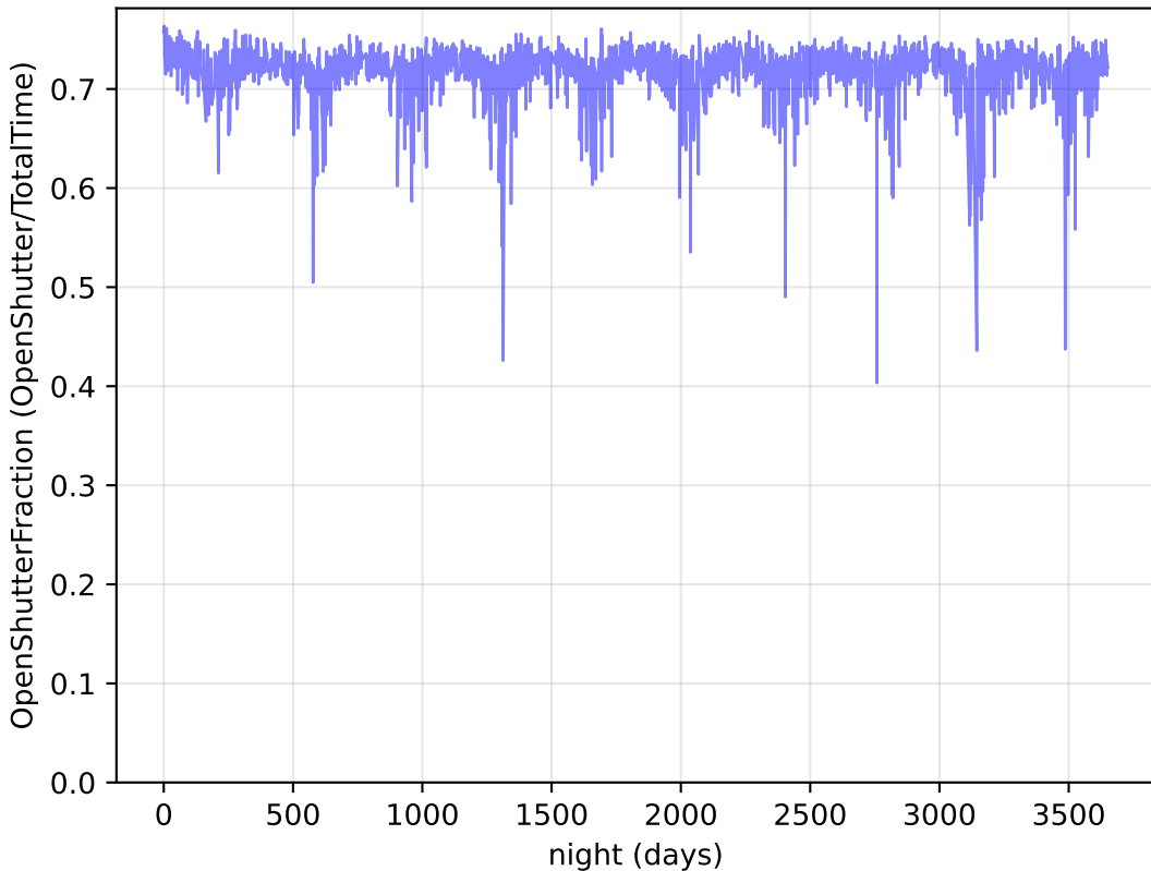
weather_cloudso16v3.4_10yrs : OpenShutterFraction
