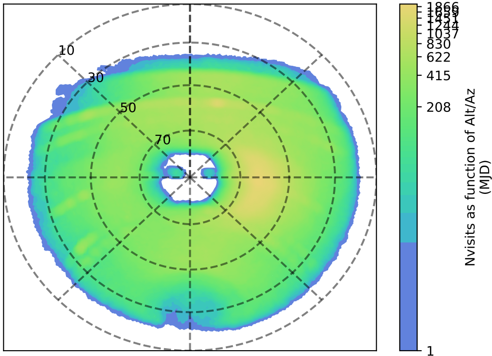
weather_cloudso16v3.4_10yrs y: Nvisits as function of Alt/Az
