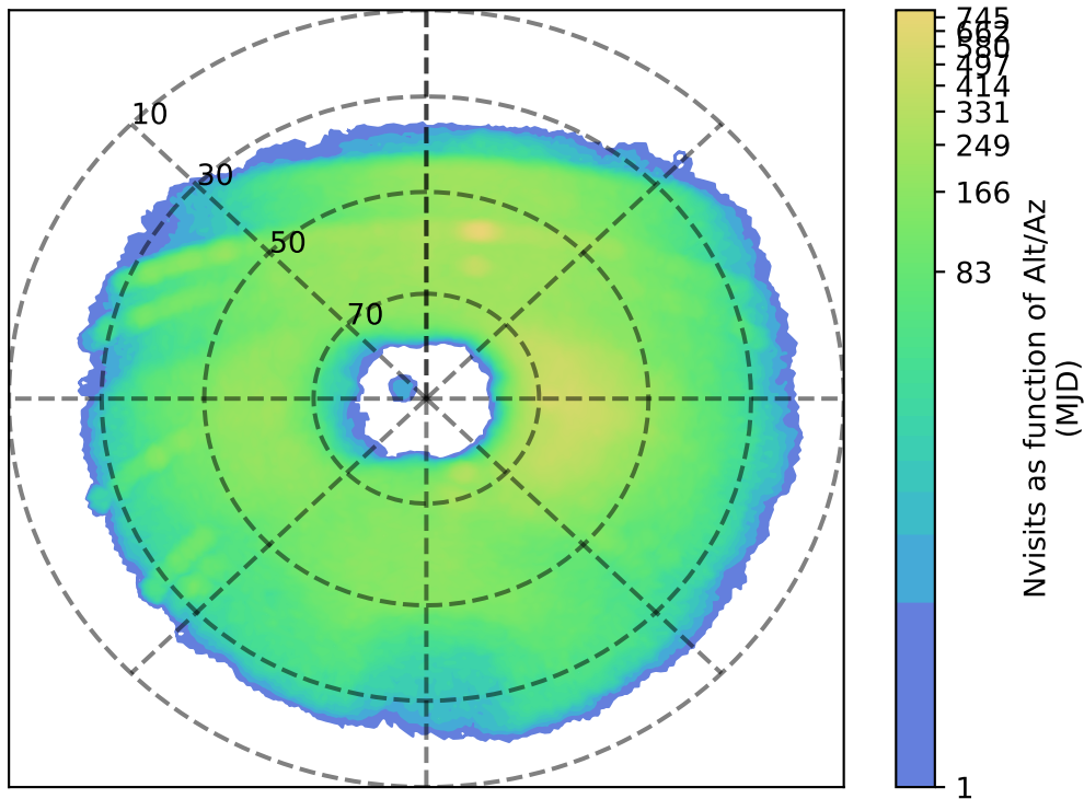
weather_cloudso16v3.4_10yrs u: Nvisits as function of Alt/Az
