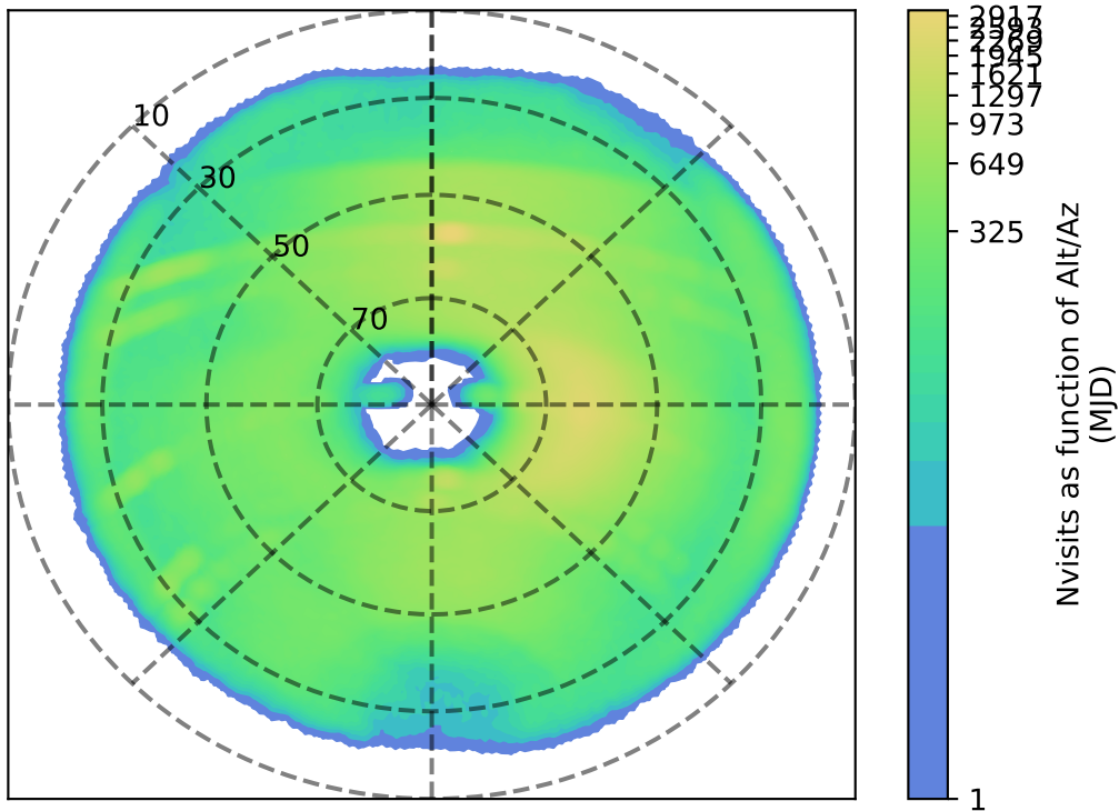
weather_cloudso16v3.4_10yrs i: Nvisits as function of Alt/Az
