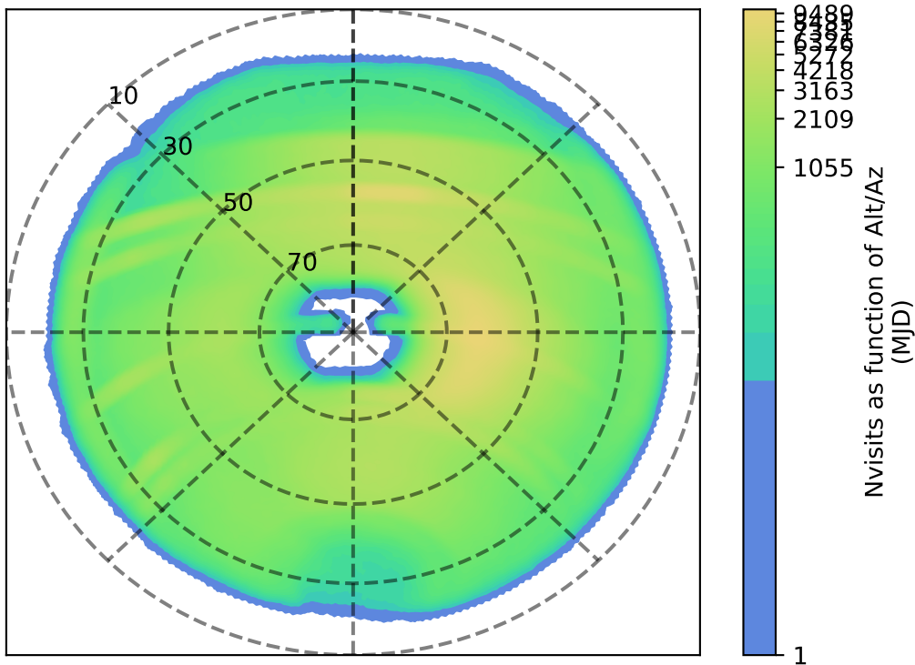
weather_cloudso16v3.4_10yrs : Nvisits as function of Alt/Az
