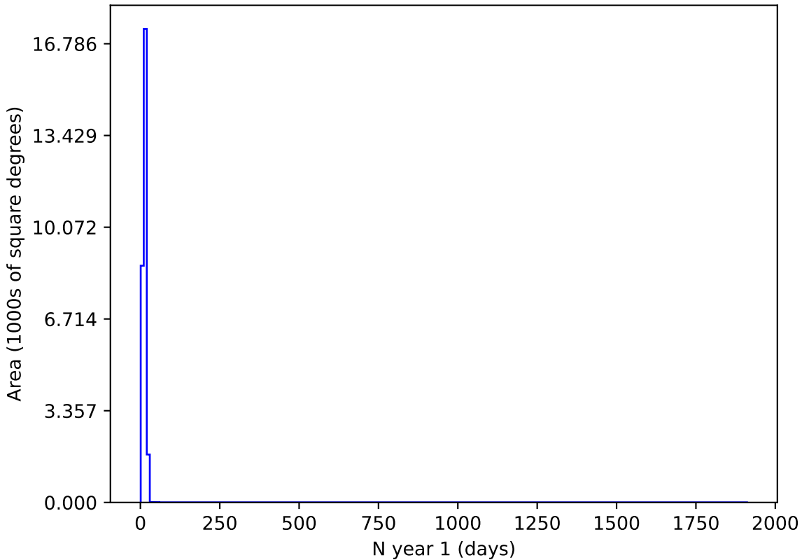
weather_cloudso16v3.4_10yrs z and night < 365: N year 1
