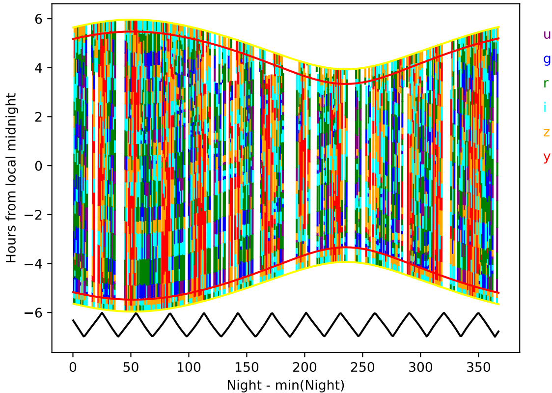
weather_cloudso16v3.4_10yrs year 7-8: Hourglass
