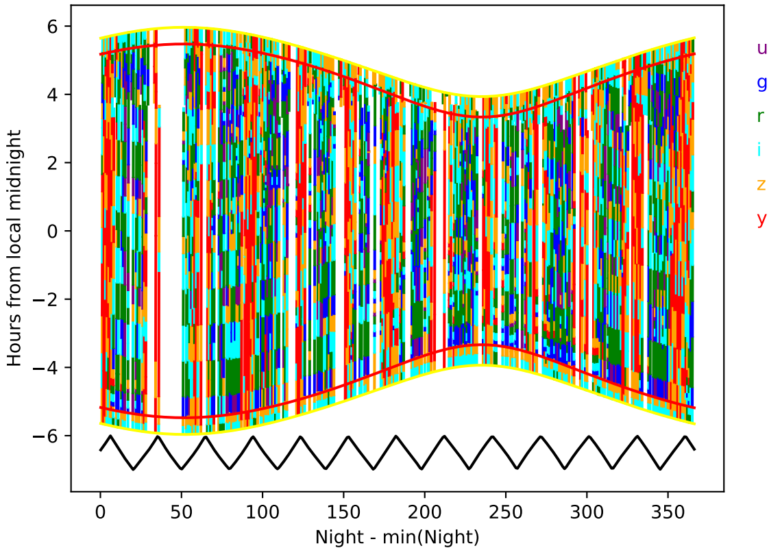
weather_cloudso16v3.4_10yrs year 6-7: Hourglass
