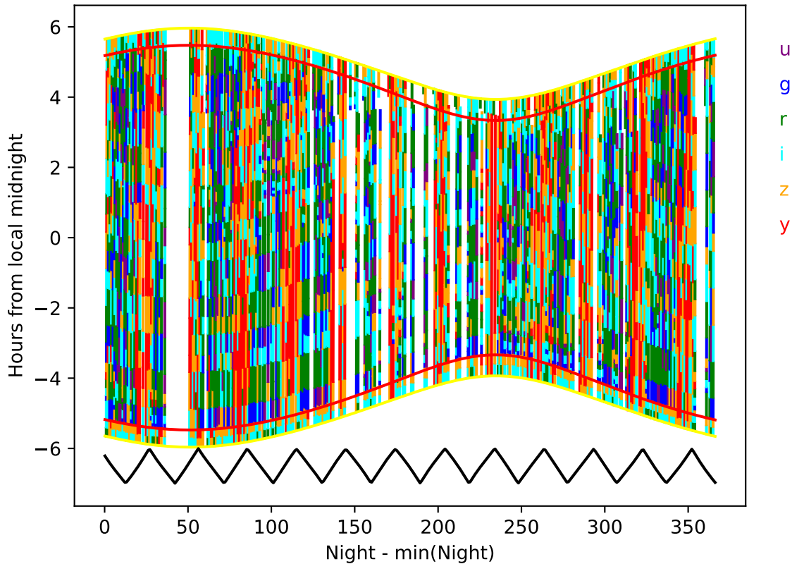
weather_cloudso16v3.4_10yrs year 4-5: Hourglass
