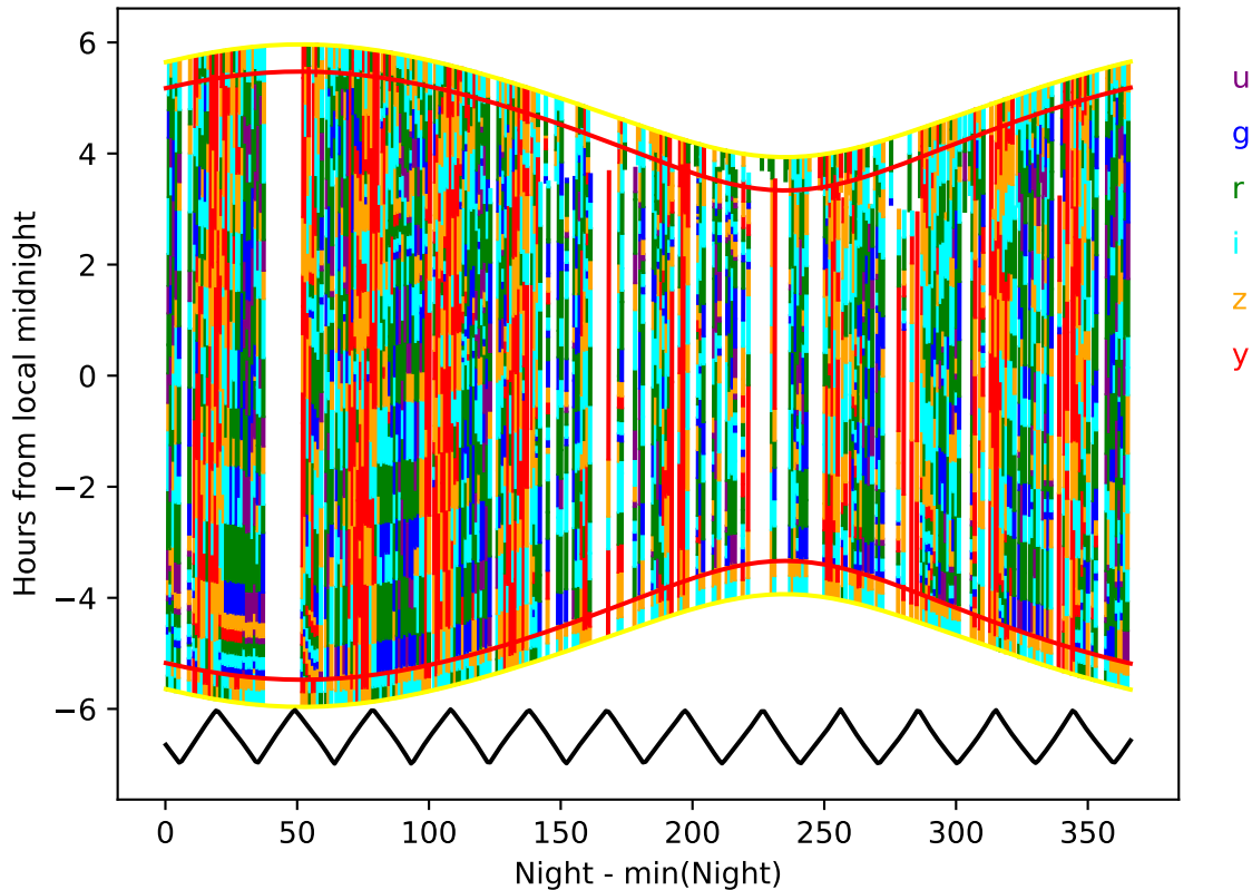
weather_cloudso16v3.4_10yrs year 2-3: Hourglass
