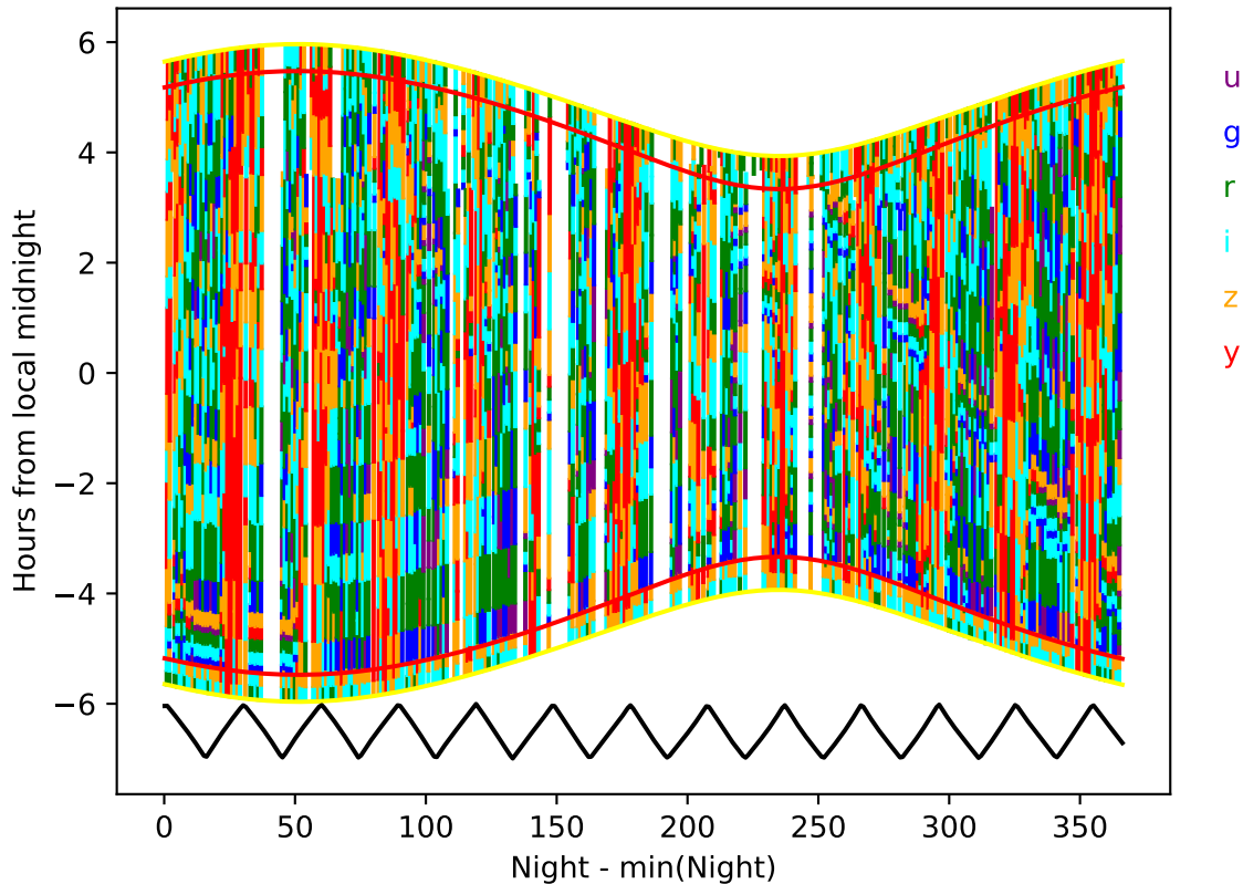
weather_cloudso16v3.4_10yrs year 1-2: Hourglass
