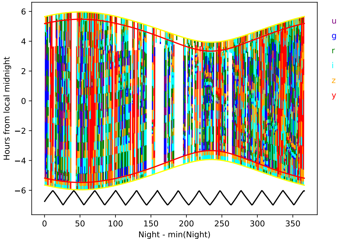
weather_cloudso16v3.4_10yrs year 0-1: Hourglass
