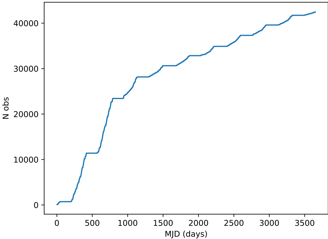
weather_cloudso16v3.4_10yrs note like DD:COSMOS%: Cumulative
