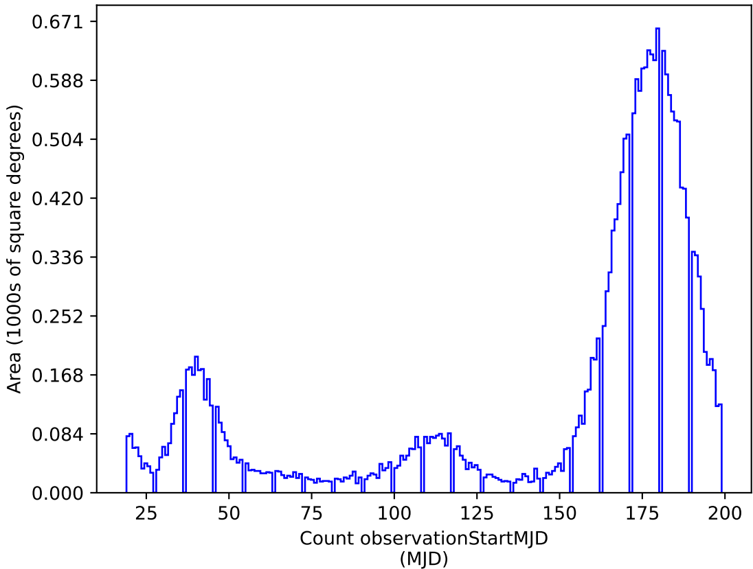
weather_cloudso16v3.4_10yrs y: Count observationStartMJD
