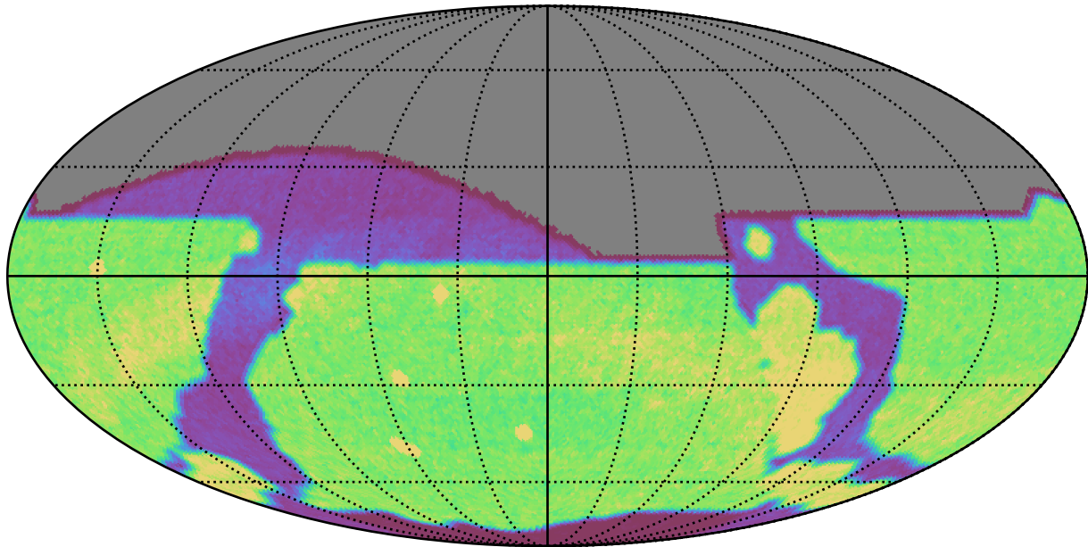
weather_cloudso16v3.4_10yrs r: Count observationStartMJD
