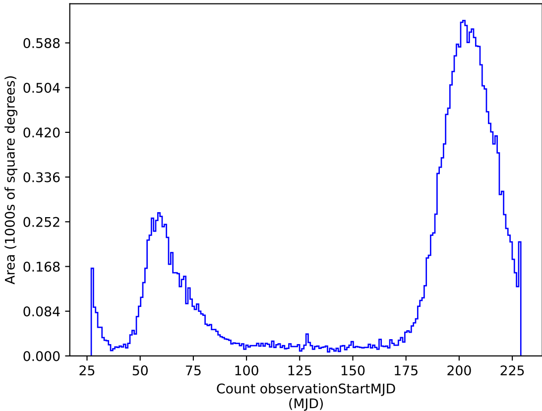
weather_cloudso16v3.4_10yrs i: Count observationStartMJD
