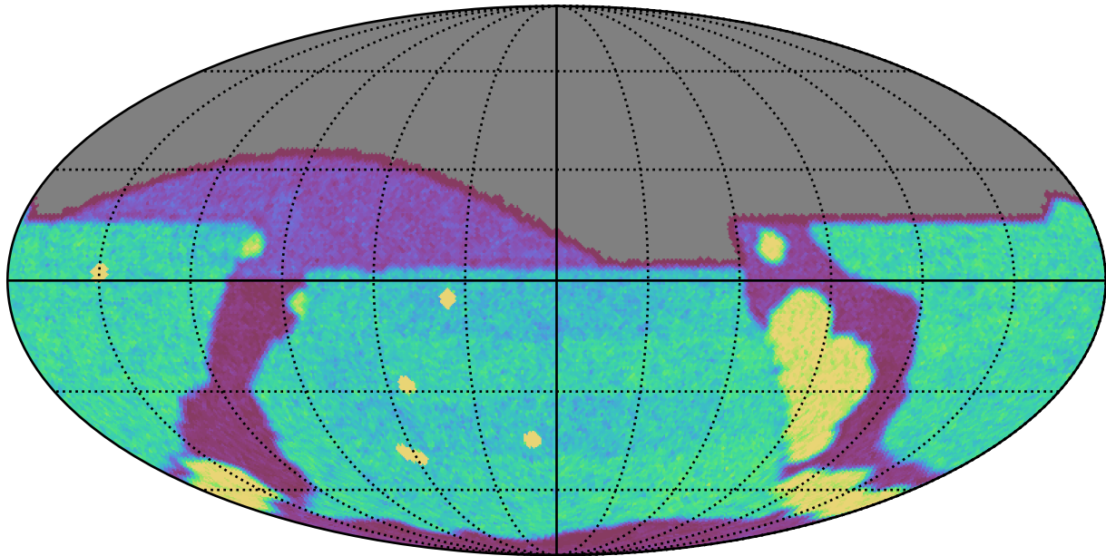
weather_cloudso16v3.4_10yrs g: Count observationStartMJD
