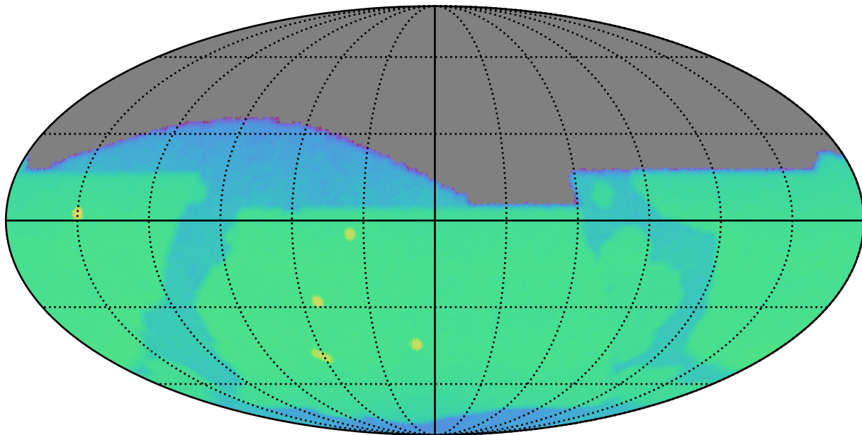
weather_cloudso16v3.4_10yrs z: CoaddM5
