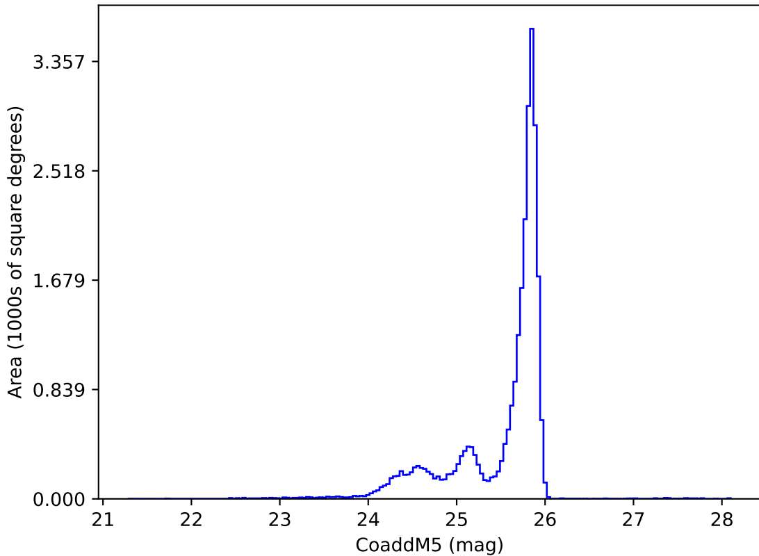
weather_cloudso16v3.4_10yrs z: CoaddM5
