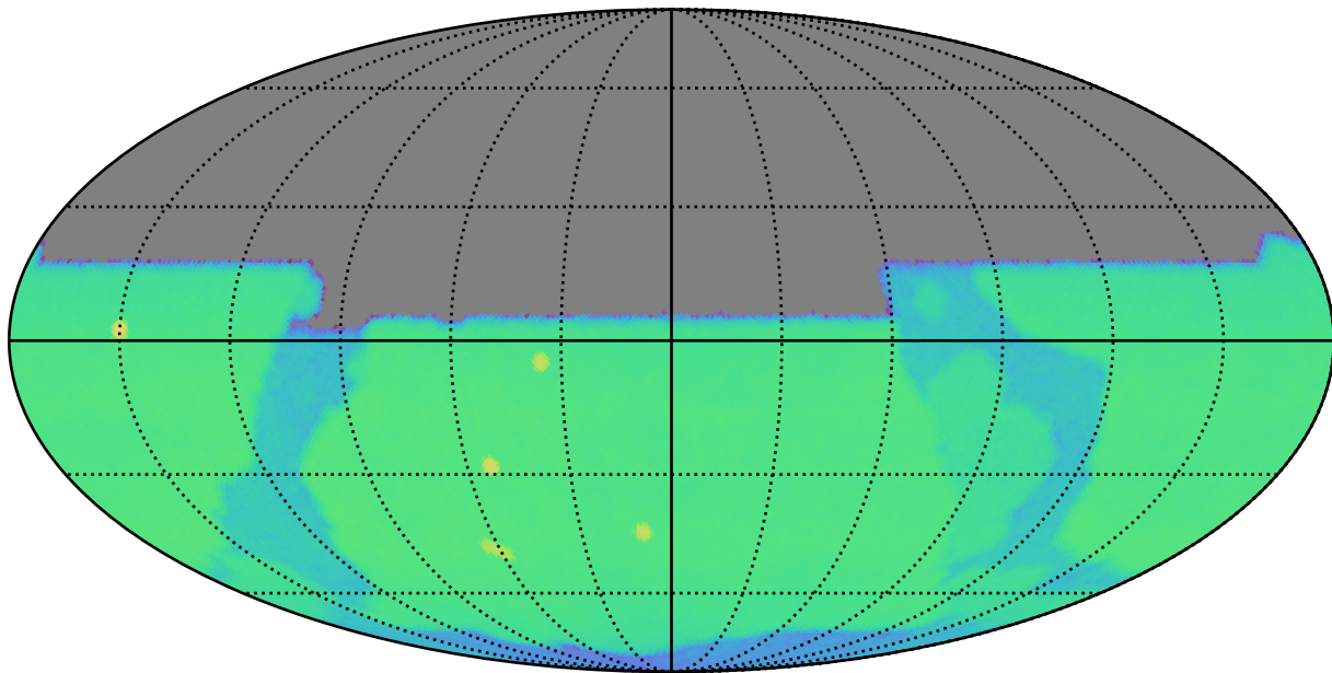
weather_cloudso16v3.4_10yrs y: CoaddM5
