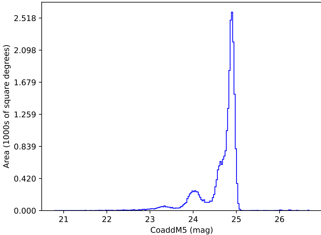
weather_cloudso16v3.4_10yrs y: CoaddM5
