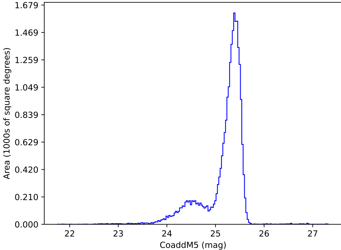
weather_cloudso16v3.4_10yrs u: CoaddM5
