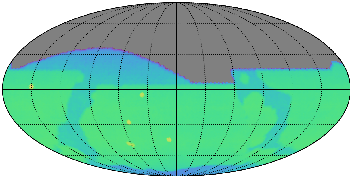
weather_cloudso16v3.4_10yrs r: CoaddM5
