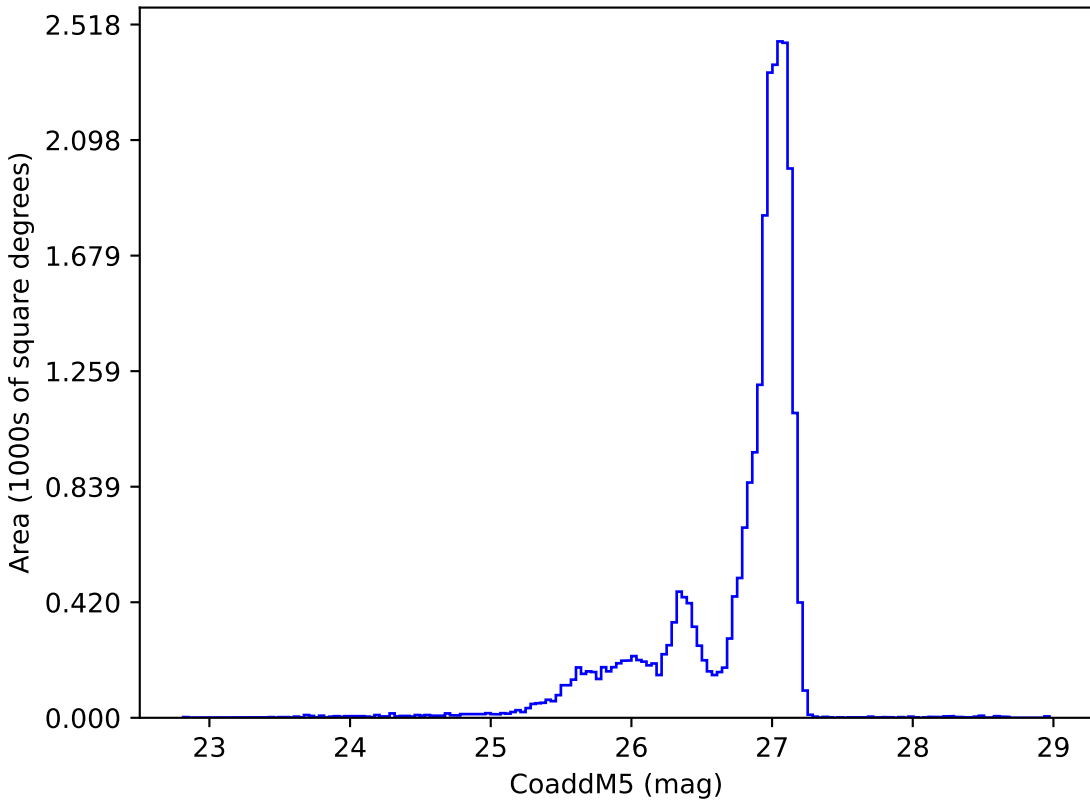
weather_cloudso16v3.4_10yrs r: CoaddM5
